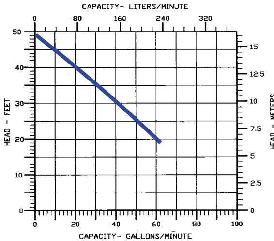
PUMP PERFORMANCE CURVE 115/60Hz
