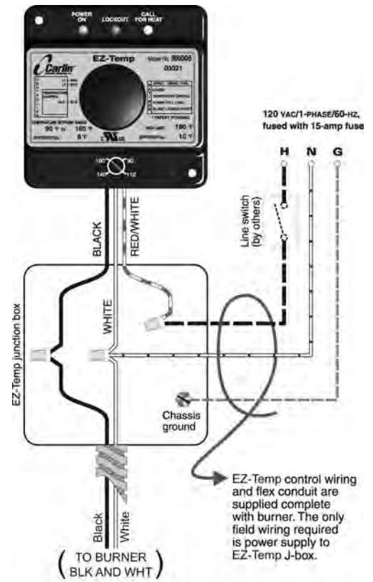
FIGURE 5: Beckett or Wayne burner w/ Carlin EZ-Temp For Models: 32, 33, 50, 51, 120
