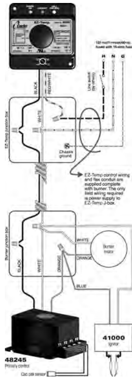
FIGURE 4: Carlin burner w/ Carlin EZ-Temp For Models: 32, 33, 50, 51, 120 (see burner manufacturer's instructions for 20e; 60200 primary w/ three wire harness)
